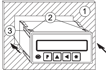
Fig. 1: Installation
