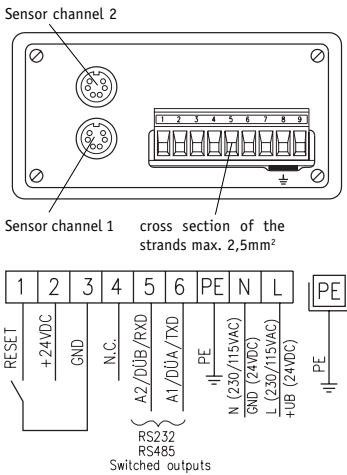
Fig. 2: Pin outs EG
