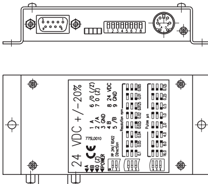
Fig. 1: Mounting / connections
