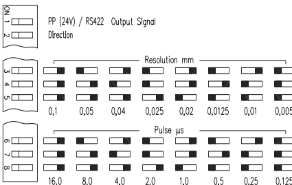
Fig. 2: DIP-switches
