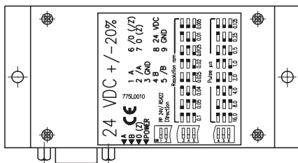
Abb. 1: Montage / Anschlüsse
