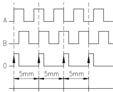
Fig. 4: Calibration principle switching length of the reference point source; REF must be <5mm!
