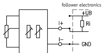
Fig. 7: Connection load against +UB
