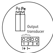
Fig. 5: Pin connection with instrument transformer
