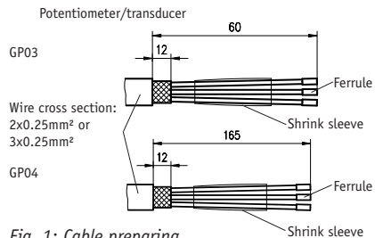
Fig. 1: Cable preparing
