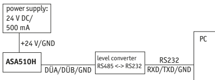
Fig. 3: Block diagram of the RS485 connection
