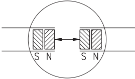
Fig. 9: Determination of the pole position. Joining the magnetic strip
