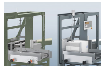
Fully automatic format adjustment through a single conversion of the manual positioning
